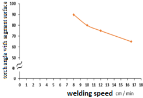
Figure 8: Chart of torch angle with segment surface at different
