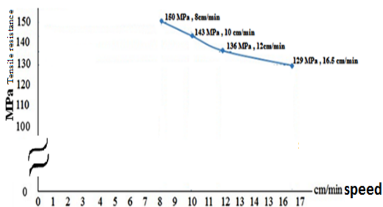
Figure 24: Effect of welding speed on final resistance of connection
