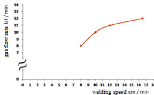
Figure 6: Chart of gas flow rate at different
