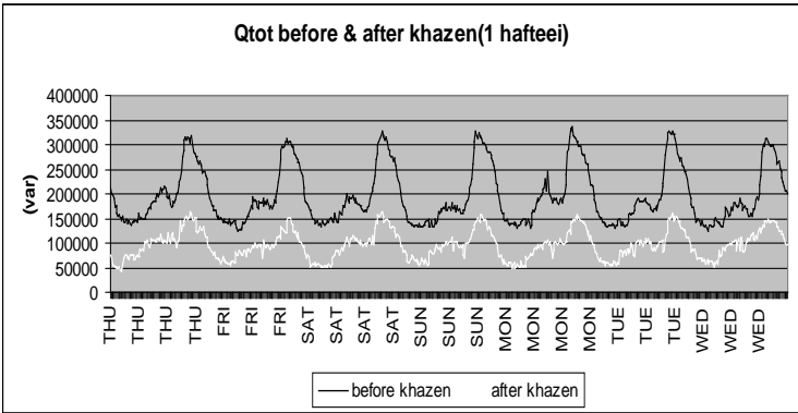
Figure 1_b) reactive power after and before capacitor placement (one week)
